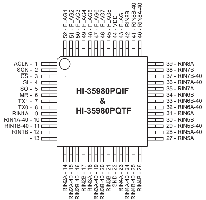
HI-35980 Full function, full pin-out version 52 - Pin Plastic Quad Flat Pack (PQFP)
