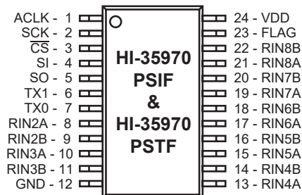
HI-35970 minimum footprint, reduced pin-out version 24 - Pin Plastic Small Outline package (SOIC)
